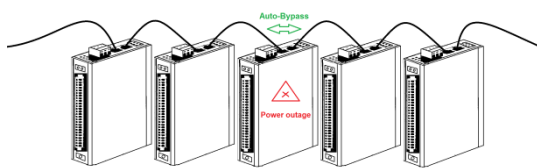
Daisy-Chain Ethernet Cabling
